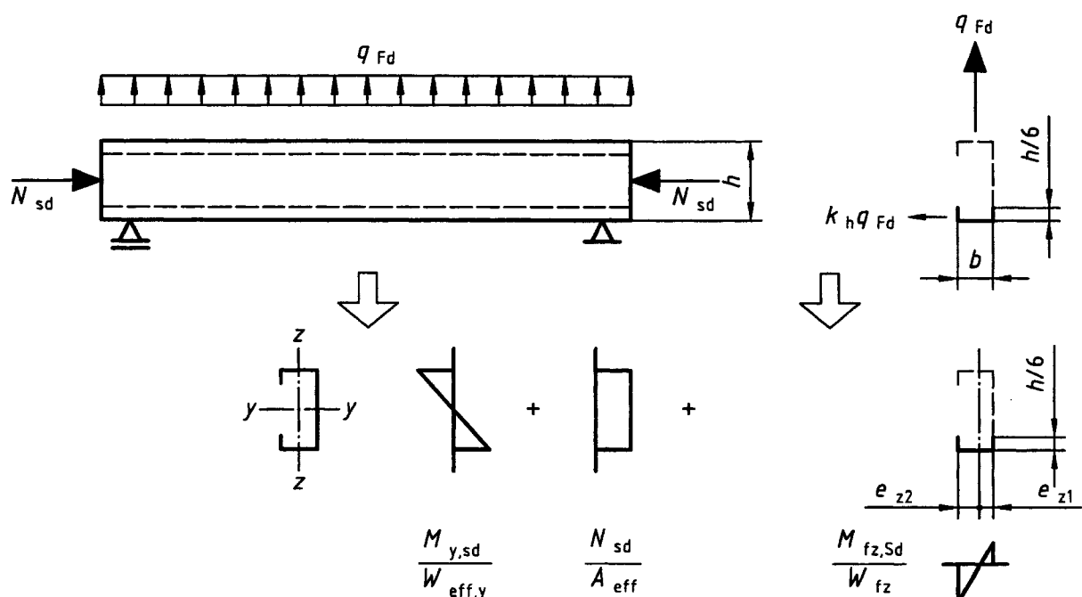
Figure 10.2 : Superposition des contraintes
